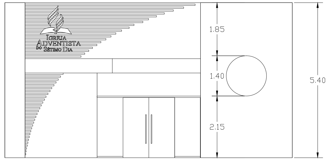
Vista Frontal
